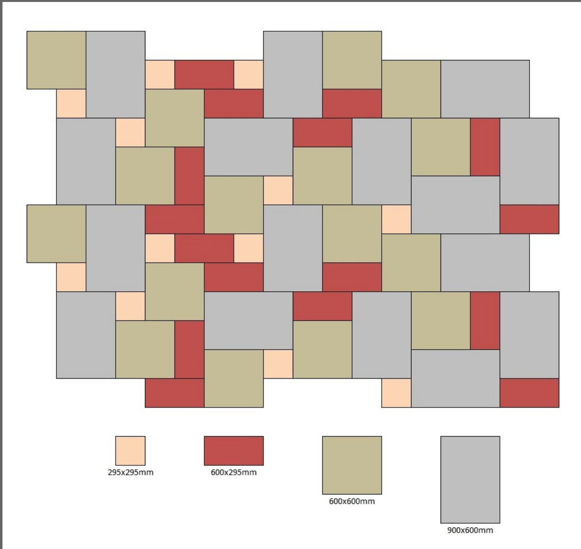
4 size paving laying pattern
